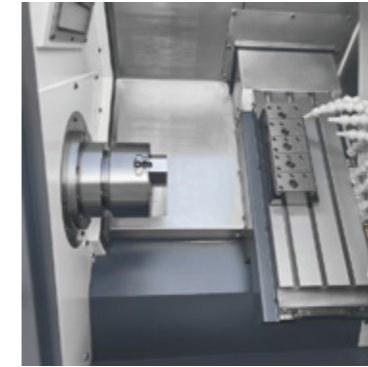
Machine inside
